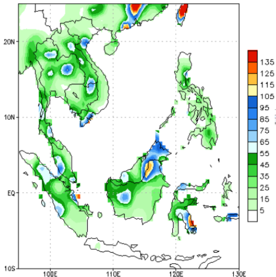
7-day Accumulated Prep (mm) 17MAY2019-23MAY2019
